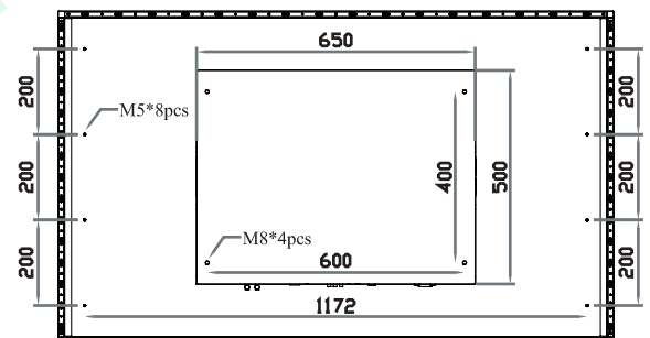
Rear View
