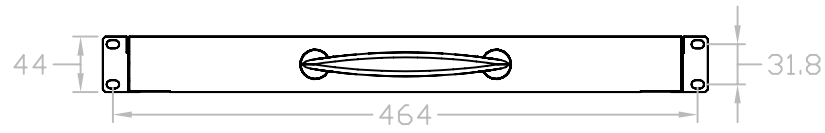
Front view
