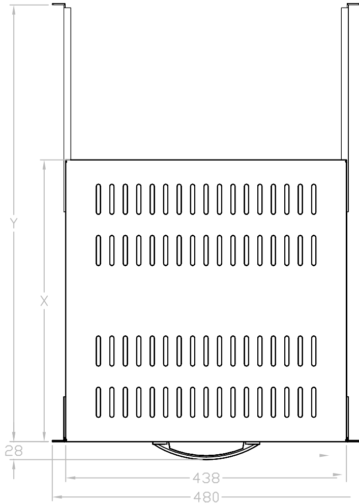
Top view
