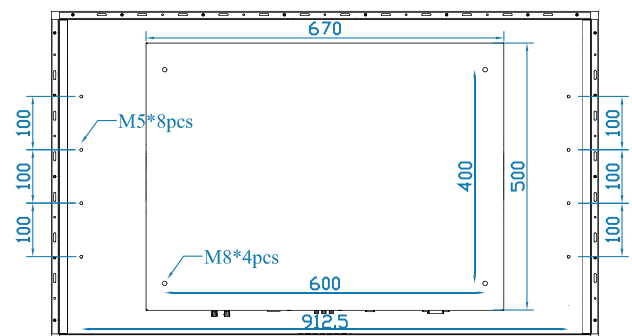
Rear View
