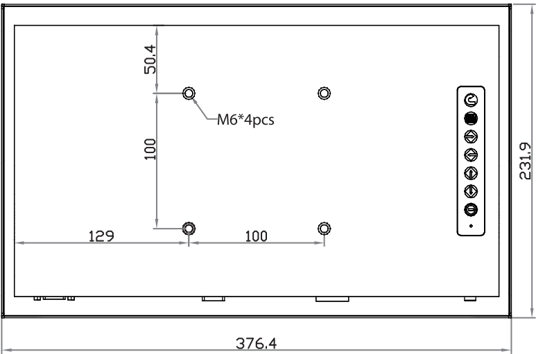
Rear View
