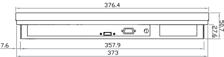
Bottom View
