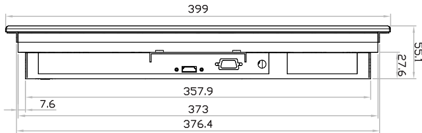
Bottom View
