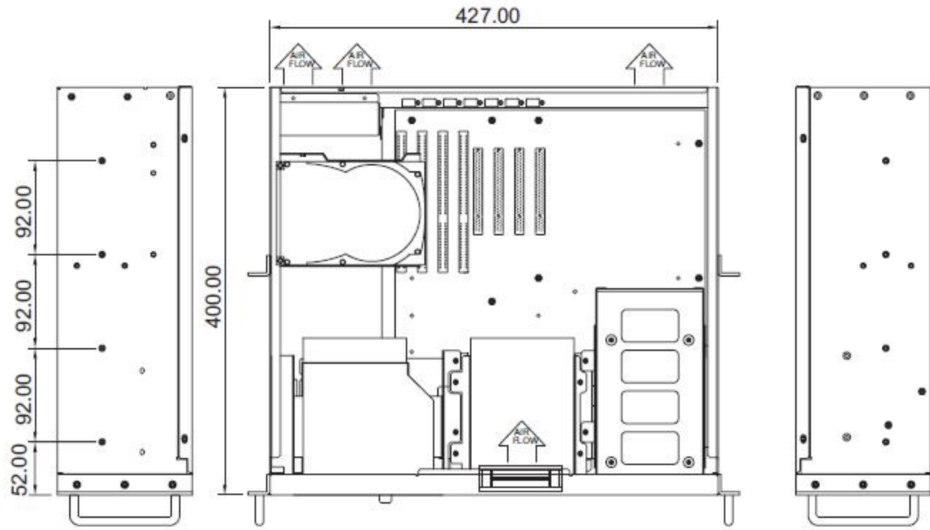
Left-side View
