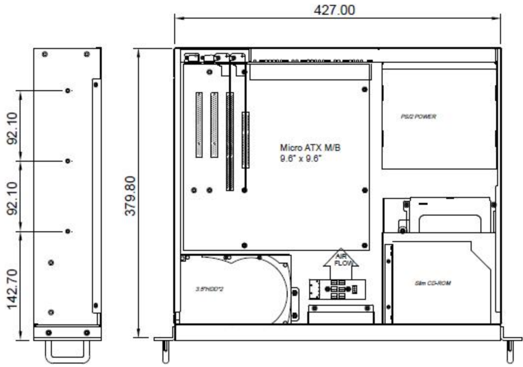
Left-side View
