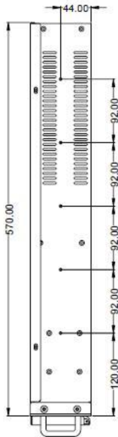
Right-side View
