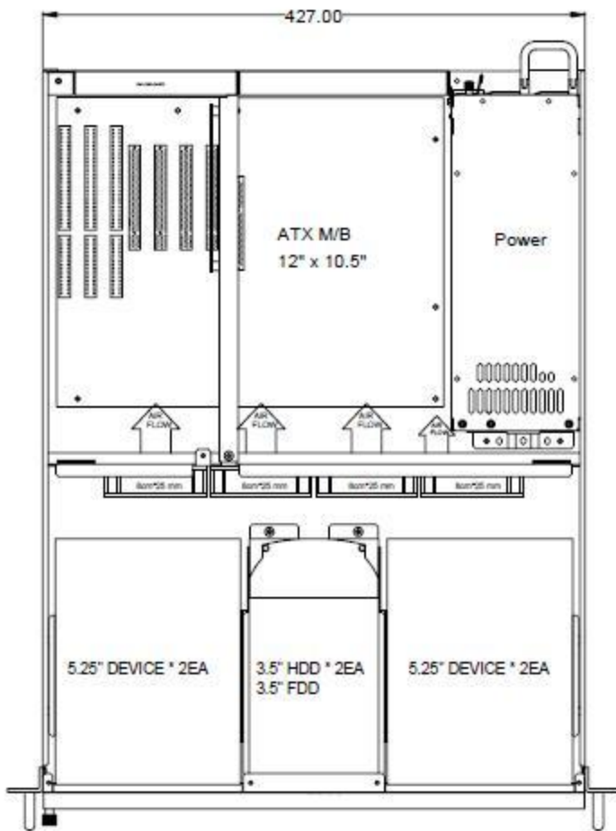
Top View
