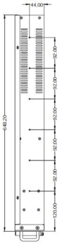
Right-side View
