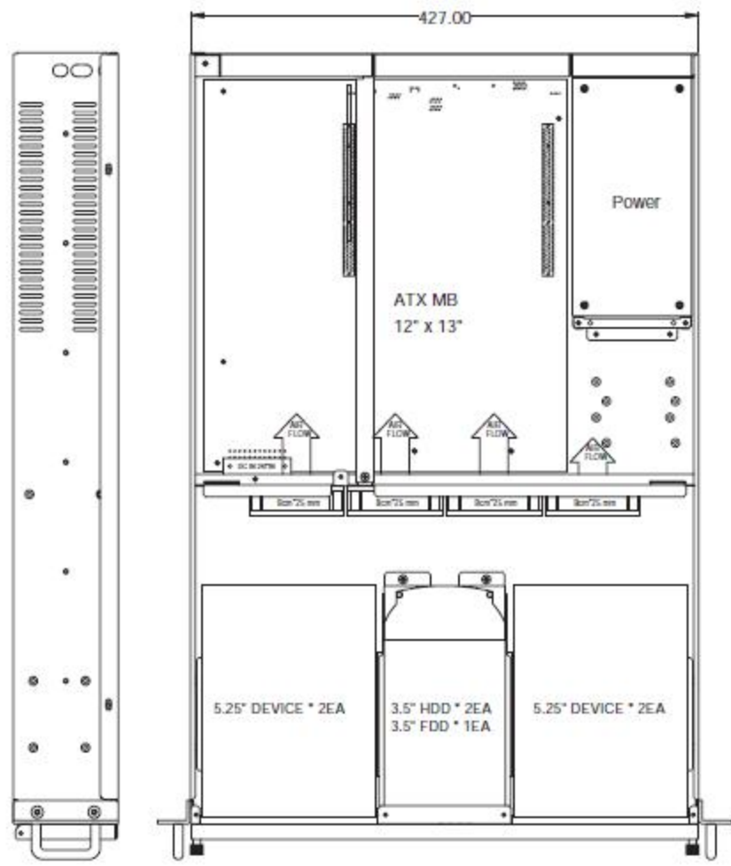
Left-side View
