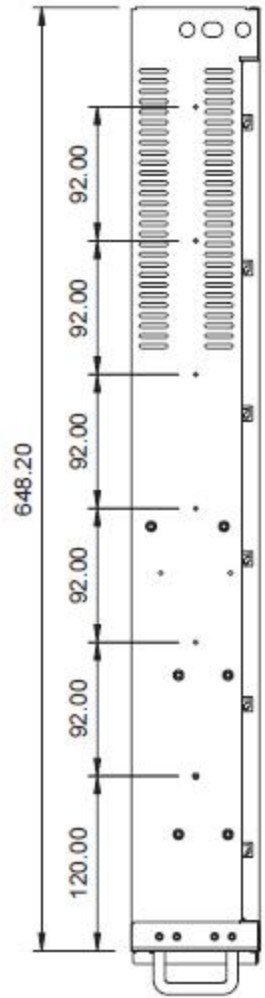
Left-side View
