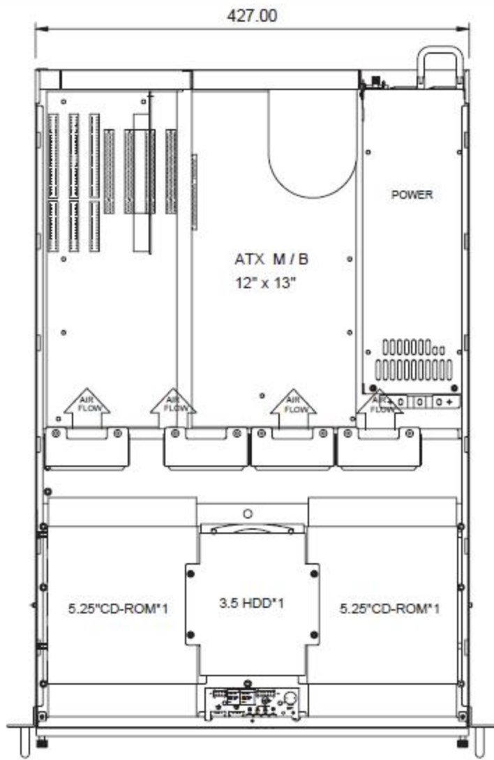
Top View
