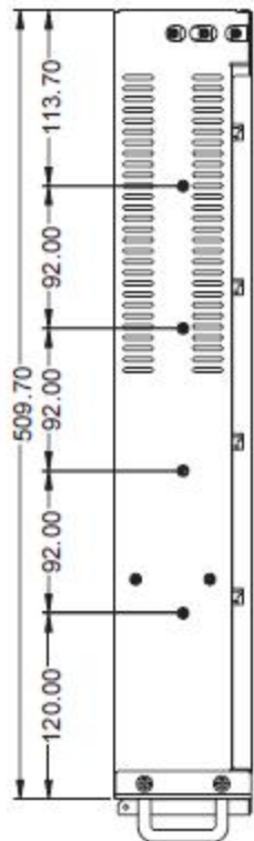
Left-side View
