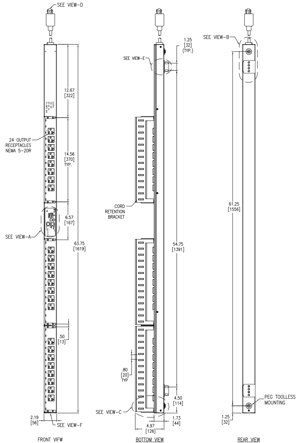
FRONT VIEW
