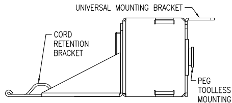
VIEW F (RIGHT SIDE VIEW-ENLARGED)
