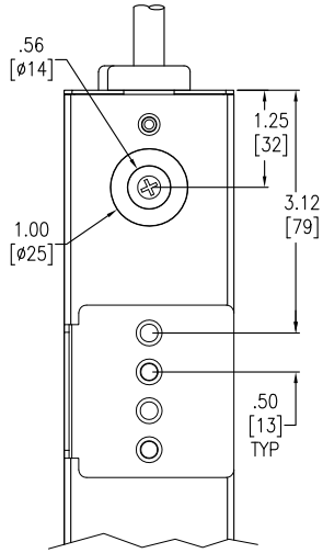
VIEW B (ENLARGED)
