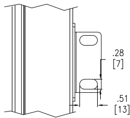
VIEW E (MOUNTING BRACKET-ENLARGED)
