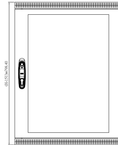
Vented Door Front view
