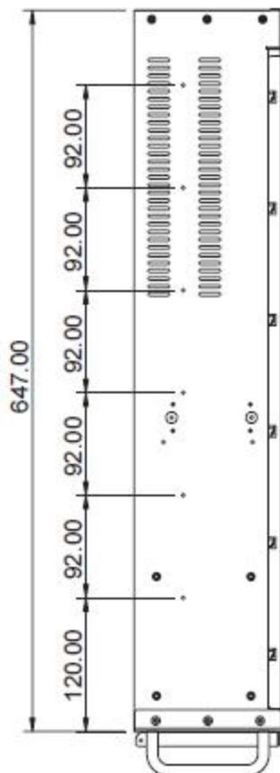
Left-side View
