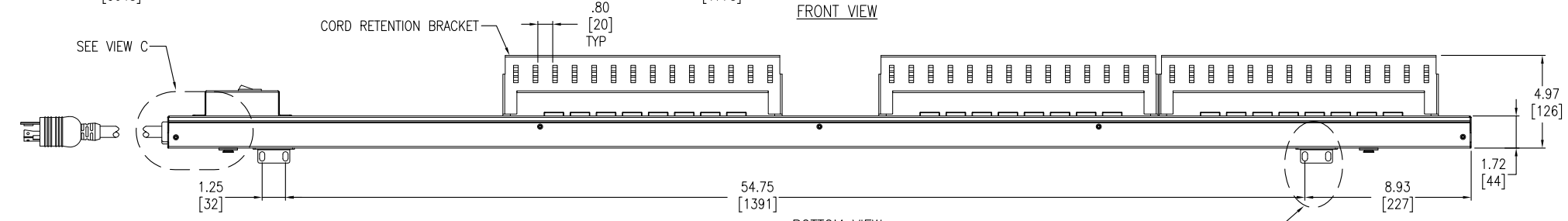
BOTTOM VIEW
