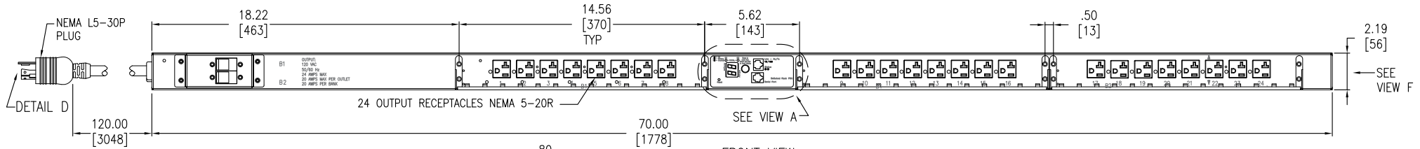
FRONT VIEW
