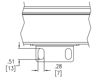
VIEW E (MOUNTING BRACKET-ENLARGED)
